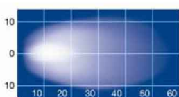
72419 Dual Purpose Flood Beam Ideal for vertical pillar (materials handling) or horizontal (agriculture) mounting
